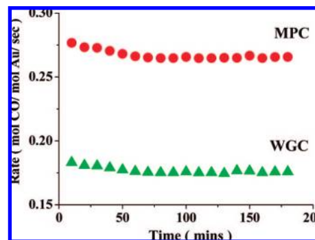
Figure 6. Change in catalytic activity over time for the WGC and MPC catalysts. Steady-state activity measurements were determined only after the rate stabilized (ca. 1 h).
